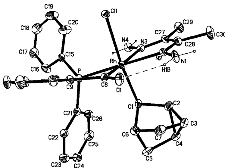
Figure 1. ORTEP view of complex 2 , showing the atomic numbering (30% probability ellipsoids); solvent molecules, some carbon atoms and all hydrogen atoms but four have been omitted for clarity; selected bond lengths [Å] and angles [°]: Rh–C(1) 2.12(2), Rh–C(8), 2.00(2), Rh–N(2) 2.10(1), Rh–N(3) 2.16(1), Rh–P 2.273(3), Rh–Cl(1) 2.525(3), O(1)–C(8) 1.21(1); C(8)–Rh–C(1) 97.8(5), C(8)–Rh–N(2) 97.9(4), C(1)–Rh–N(2) 89.2(4), C(8)–Rh–N(3) 170.7(4), C(1)–Rh–N(3) 87.8(4), N(2)–Rh–N(3) 74.7(4), C(8)–Rh–P(1) 83.2(3), C(1)–Rh–P(1) 90.1(3), N(2)–Rh–P 178.8(3), N(3)–Rh–P 104.3(3), C(8)–Rh–Cl(1) 85.2(3), C(1)–Rh–Cl(1) 174.2(4), N(2)–Rh–Cl(1) 85.5(3), N(3)–Rh–Cl(1) 88.6(3), P(1)–Rh–Cl(1) 95.2(1).
