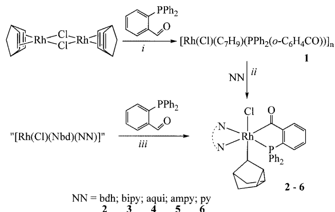
Scheme 1. Formation of nortricyclyl derivatives in benzene.
