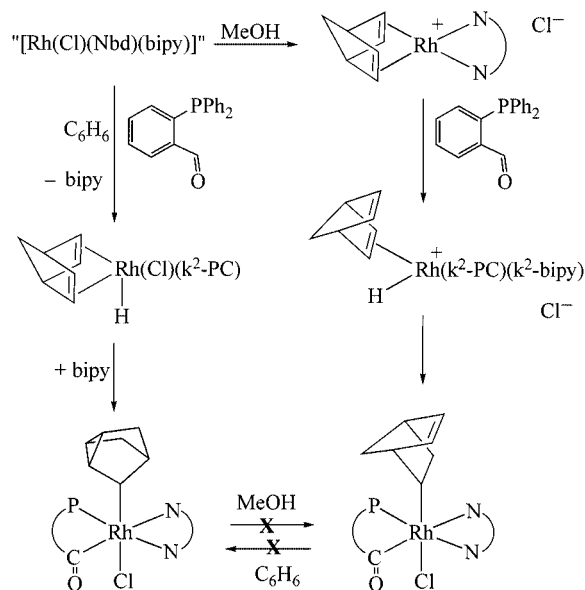
Scheme 2. Proposal for the selective production of nortricyclyl and norbornenyl derivatives.
