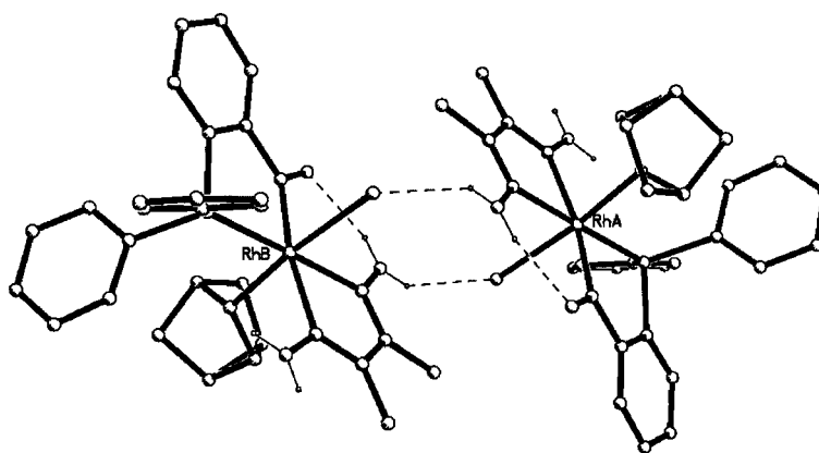
Figure 2. PLUTO view of the “dimer units” showing the hydrogen bonds for 2 .
